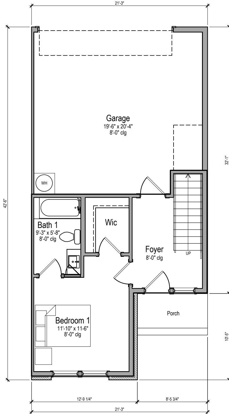
First Floor Floor square footage: 388 sq. ft.
