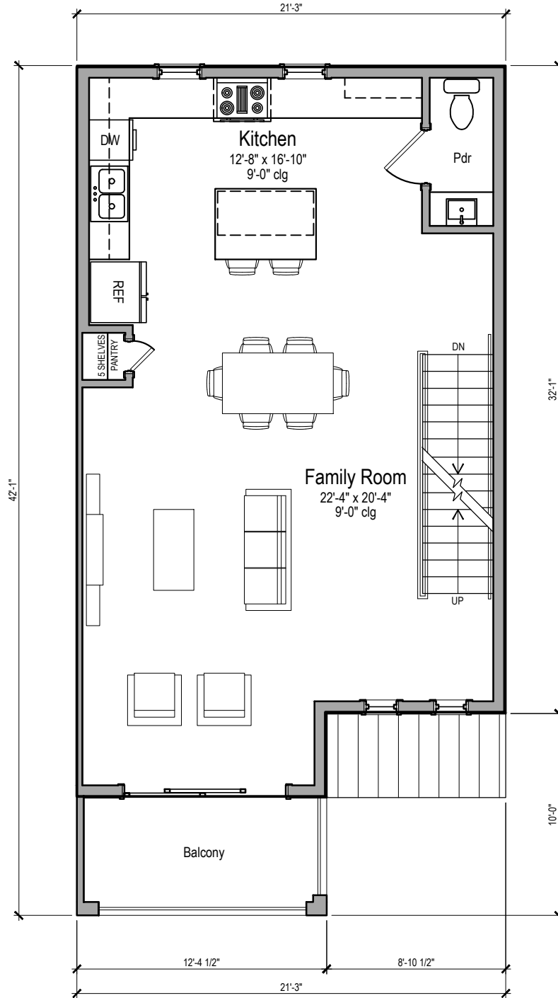
Second Floor Floor square footage: 728 sq. ft.
